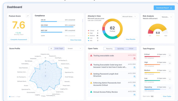
Cynomi Security Dashboard
